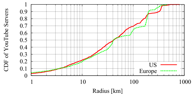
Fig. 3. Radius of the CBG confidence region for the YouTube servers found in the datasets.
