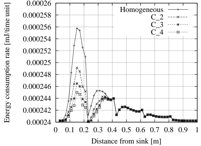
Figure 5. Average energy consumption rate per sensor as a function of the node distance from the sink, under different network deployments
