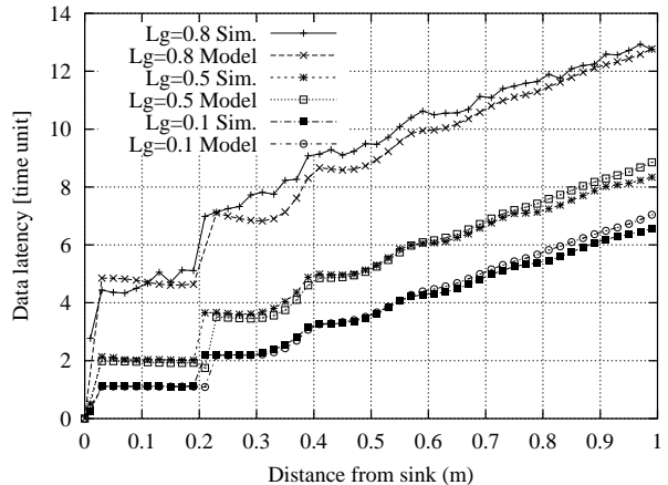
Figure 3. Average data latency vs. the node distance from the sink, for different values of L_g . Analytical and simulation results are compared
