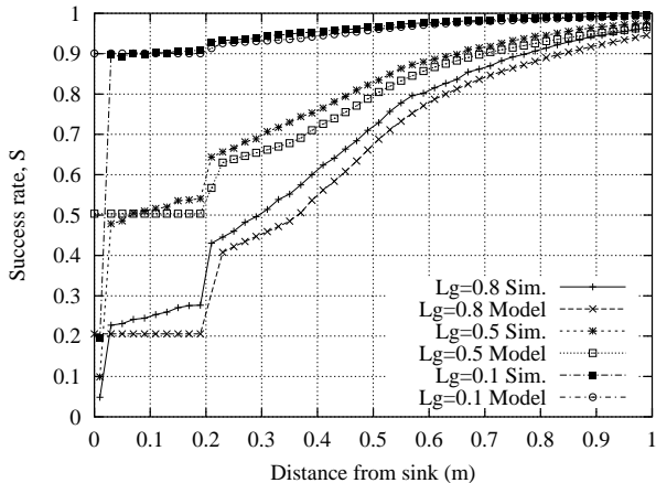
Figure 2. Success rate per sensor as a function of the node distance from the sink, for different values of L_g . Analytical and simulation results are compared
