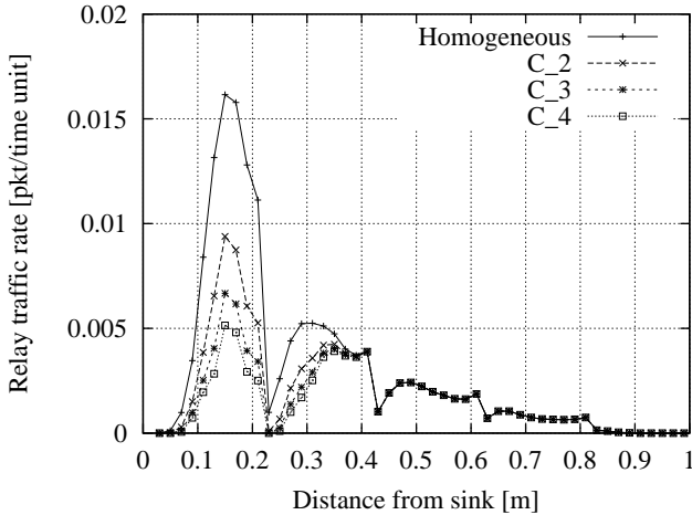
Figure 4. Average relay traffic rate per sensor versus the node distance from the sink, under different node deployments
