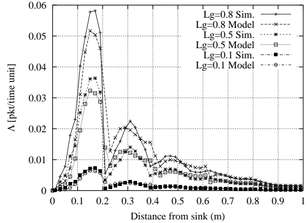
Figure 1. Average total traffic rate per sensor, \Lambda , versus the node distance from the sink, for different values of L_g . Analytical and simulation results are compared
