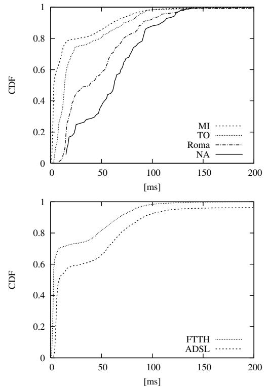
Fig. 9. CDF of RTT from different Cities on the top, and versus network access on the bottom.
