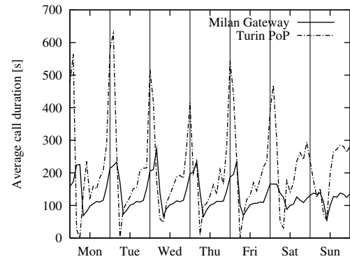
Fig. 7. Average phone call duration versus time.
